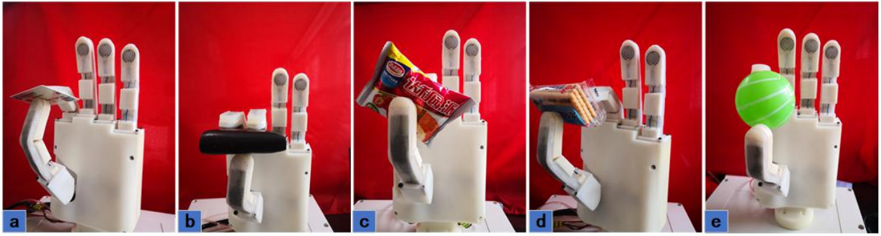
Fig.13. Experiments of pinching different objects
