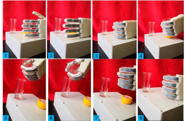
Fig.17. Demonstration of pouring water
