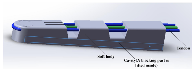
Fig.1 . Prototype of the soft finger with variable stiffness
