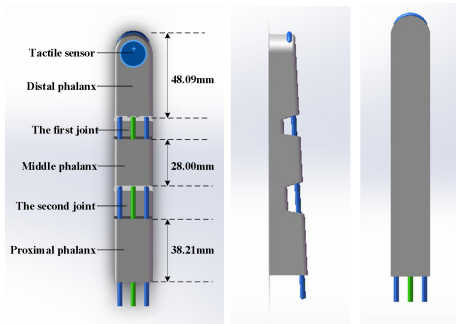
Fig.4. Prototype of the index finger
