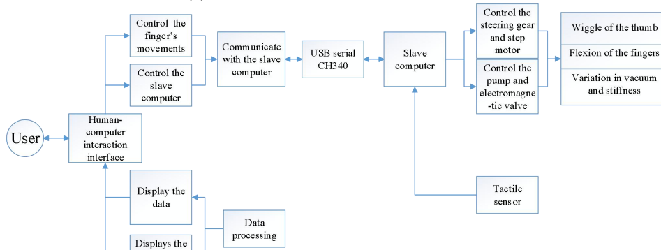
Fig.8. Control strategy of the SHH-VS system
