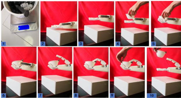
Fig.14. Demonstration of bowl(500g)being held in the palm
