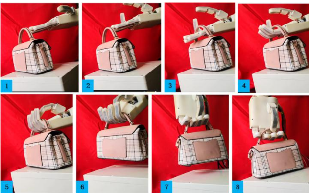
Fig.15. Demonstration of the handbag being lifted
