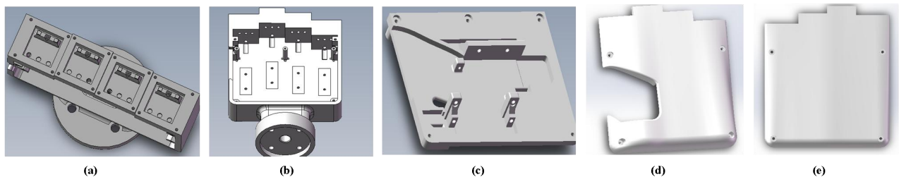
Fig.7. The structure of the palm. (a) The rabbet of the distal phalanx. (b) The internal structure of the palm.(c) The support plate of the thumb.(d) The front of the palm.(e) The back of the palm.
