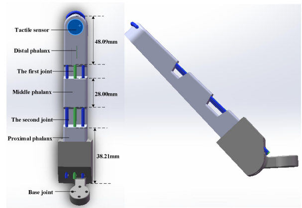
Fig.6. Prototype of the thumb finger
