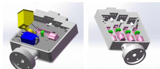
Fig.2. Prototype of the SHH-VS assembled with five soft fingers
