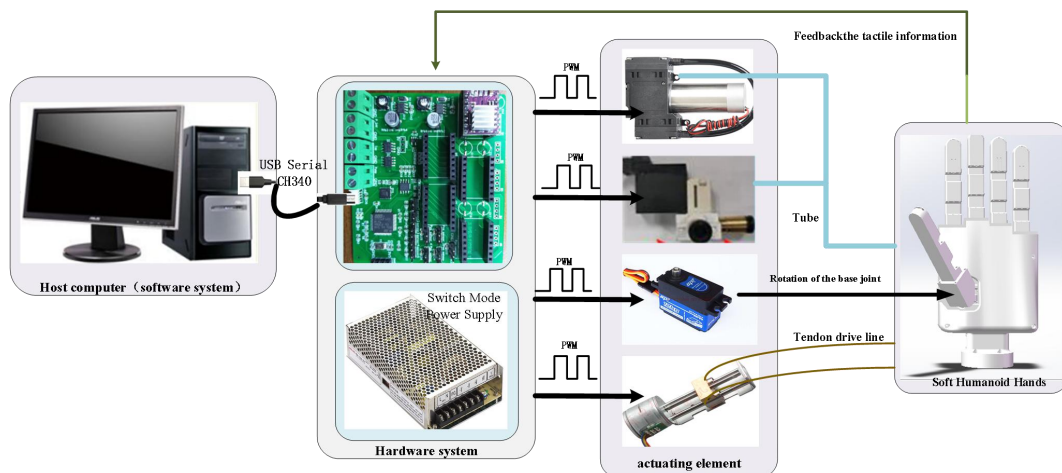
Fig.9. Hardware connection of the SHH-VS control system
