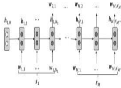
Fig-2 LSTM Prediction Model
