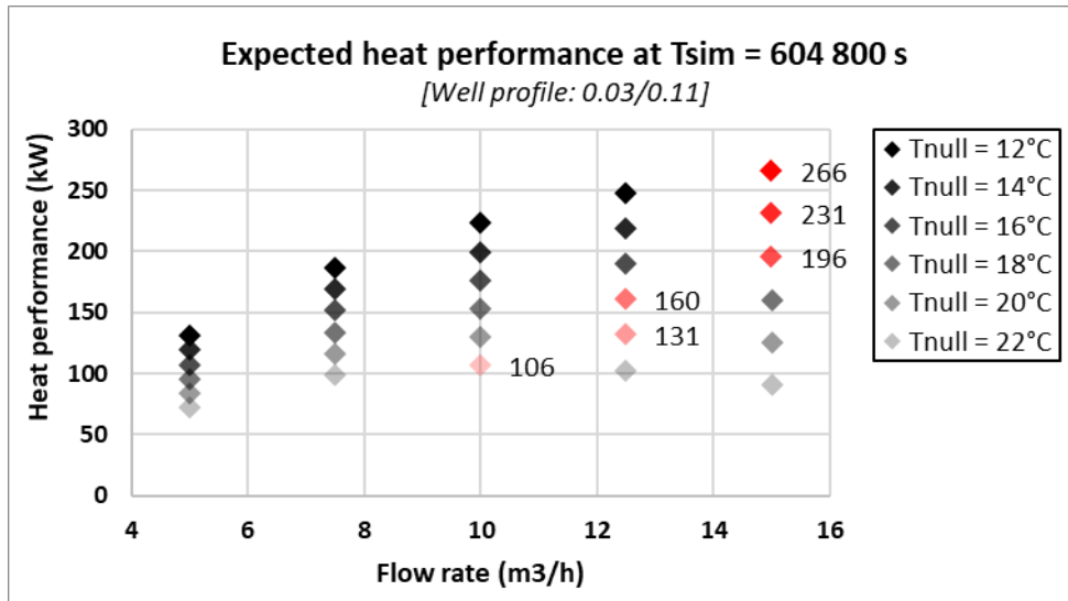
Figure 2.: Performance calculated from flowline temperature for each simulation. Maximum values, marked with red diamonds indicate that peak performance drops with reduced dT (valid for a specific timestep, under constant temperature injection).
