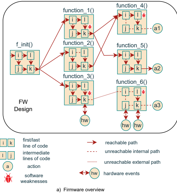
Fig. 2. Methodology for the detection of unreachable paths and weaknesses detection based on CBMC and Python scripts in FW designs
