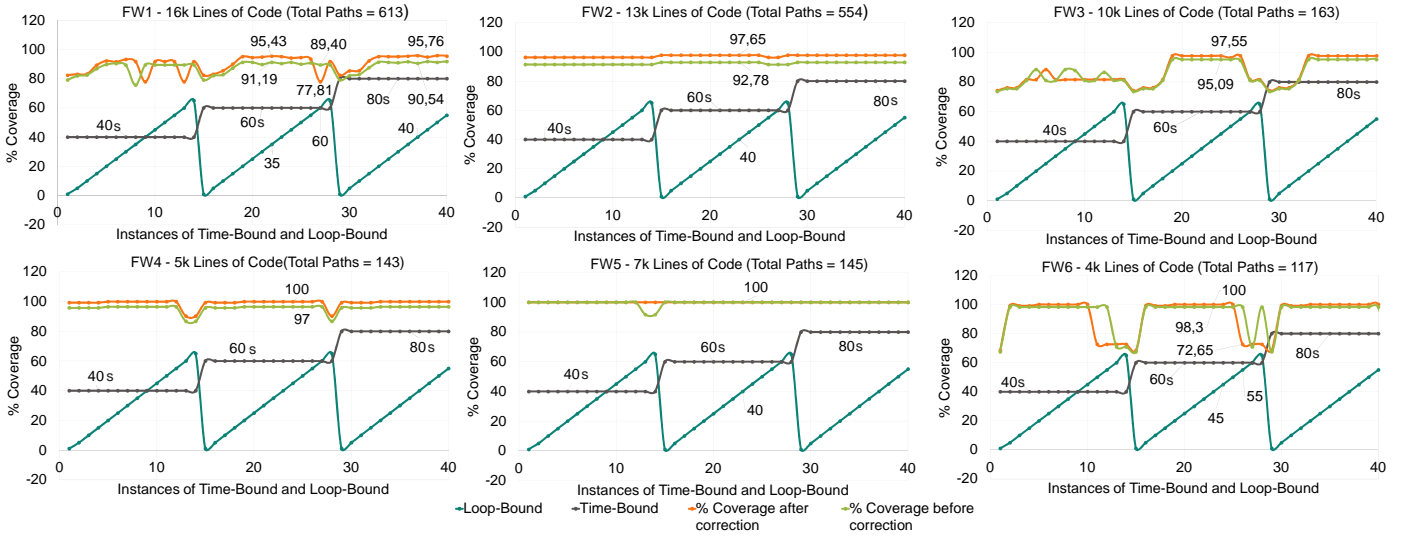
Fig. 3. % Code coverage before and after the correction of the unreachable paths
