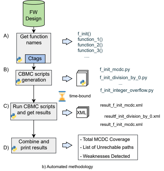
Fig. 2. Methodology for the detection of unreachable paths and weaknesses detection based on CBMC and Python scripts in FW designs
