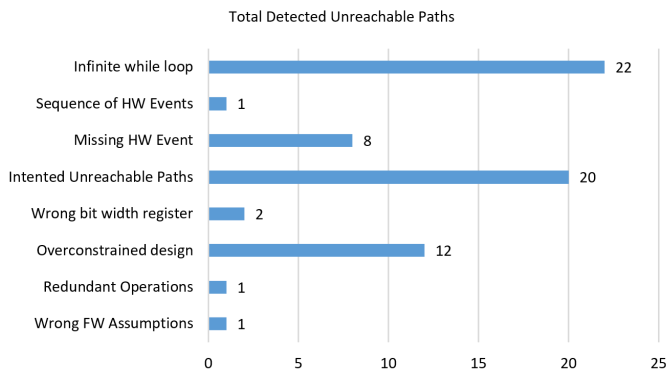
Fig. 4. Weaknesses Detection Classification
