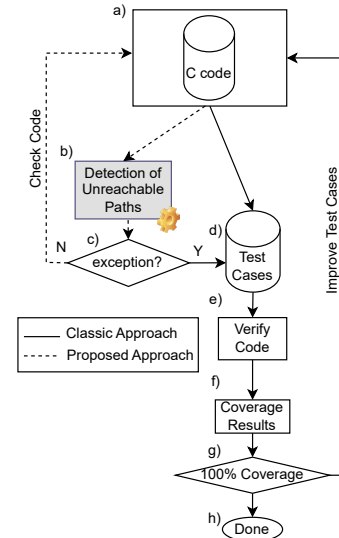
Fig. 1. Tool chain for code coverage
