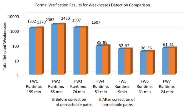
Fig. 5. Weaknesses detected before and after correction of unreachable paths
